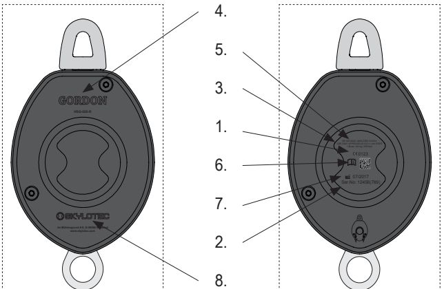
Abb. 2: HSG-020-R GORDON RESCUE
